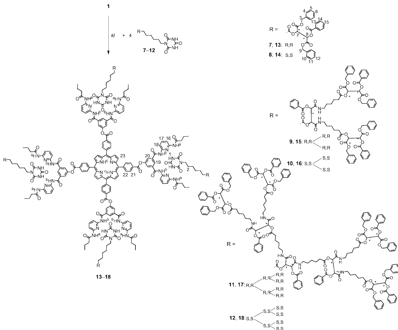
Scheme 2. General procedure for the synthesis of 13-18 : a) \text{CHCl}_3 , room temperature, 16 h.
