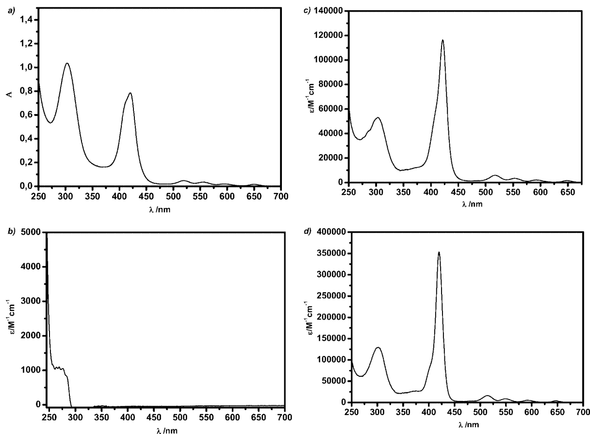
Figure 3. UV/Vis spectra: a) compound 1 in \text{CHCl}_3 (qualitative); b) compound 9 in \text{CHCl}_3 ; c) complex 13 in \text{CHCl}_3 ; d) compound 1 in THF.
