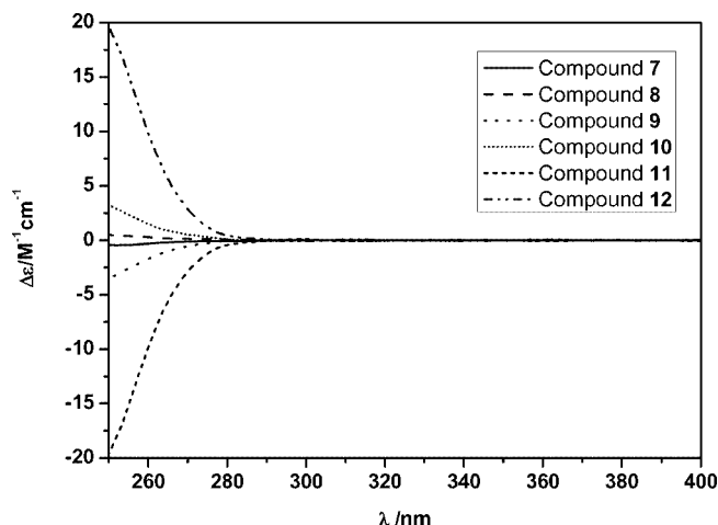
Figure 4. Circular dichroism (CD) spectra of the chiral depsipeptide dendrons 7–12 in \text{CHCl}_3 at 25 °C.
