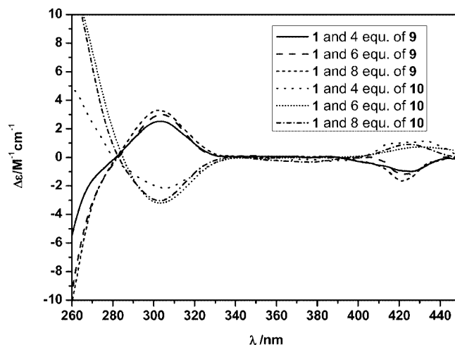
Figure 5. Circular dichroism (CD) spectra of the receptor 1 with 4–8 equiv. of the second-generation dendrons 9 and 10 in \text{CHCl}_3 at 25 °C.
