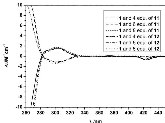
Figure 6. Circular dichroism (CD) spectra of the receptor 1 with 4–8 equiv. of the third-generation dendrons 11 and 12 in \text{CHCl}_3 at 25 °C.
