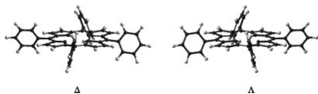
Figure 7. PM3-calculated [29] model of the C 4 -symmetric propeller-shaped tetraphenylporphyrin with \Delta and \Lambda configurations.
