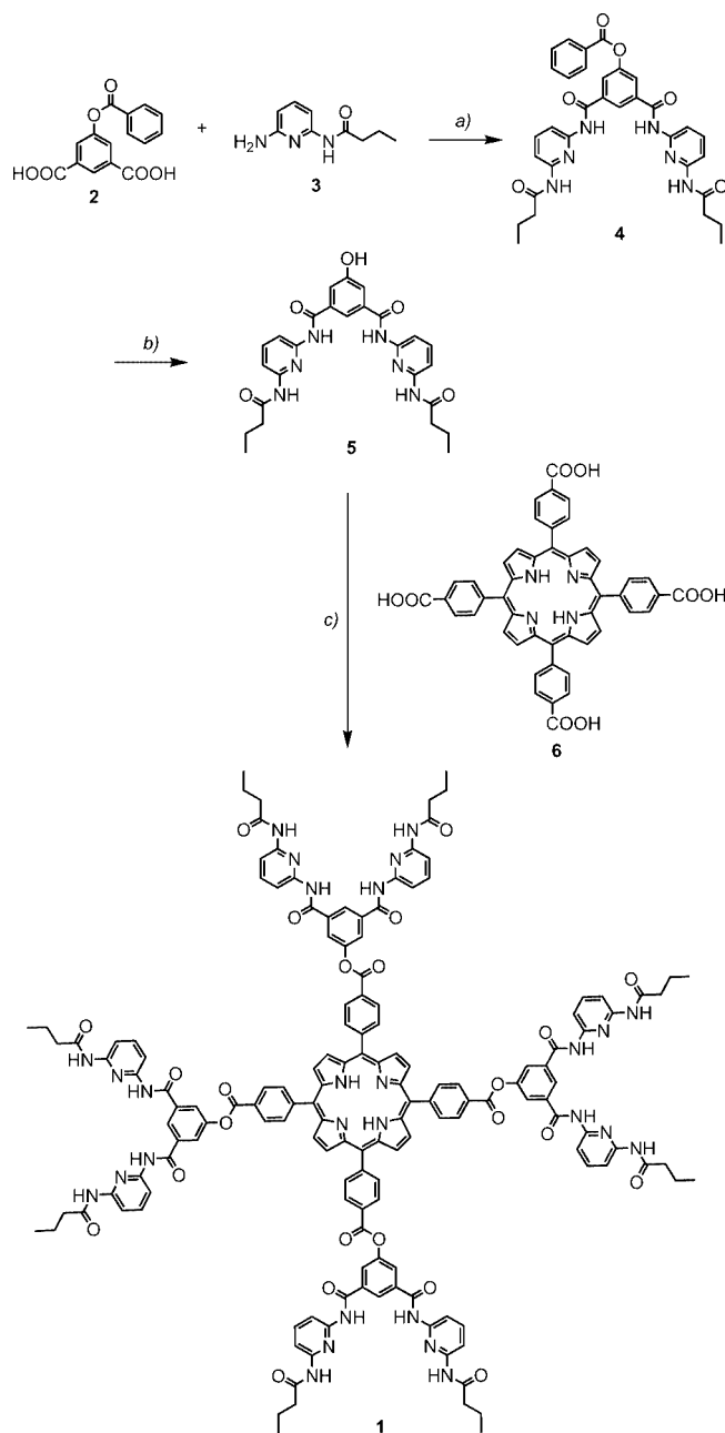
Scheme 1. Synthesis of the Hamilton receptor substituted porphyrin 1 : a) \text{SOCl}_2 , DMF, THF, room temperature, 16 h, 34%; b) KOH, dioxane, room temperature, 48 h, 61%; c) EDC, DMAP, DMF, room temperature, 7 d, 5%.
