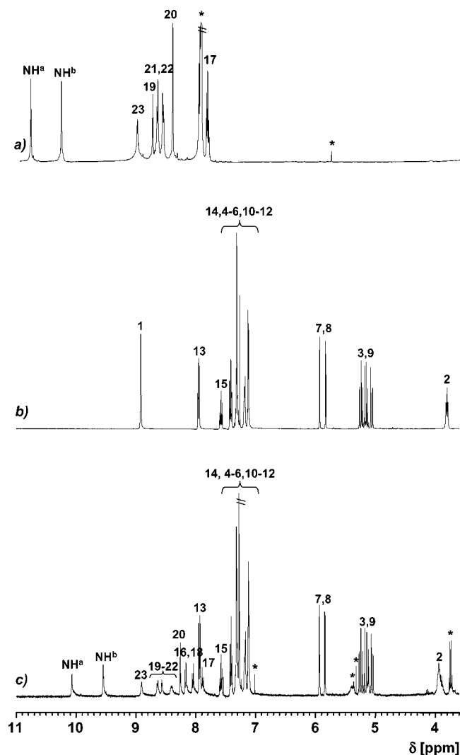
Figure 2. ^1\text{H} NMR spectra ( \delta = 3.6\text{--}11.0 ppm region, 400 MHz, room temperature): a) porphyrin derivative 1 ( [\text{D}_7]\text{DMF} ); b) depsipeptide dendron 7 ( \text{CDCl}_3 ); c) its corresponding complex 13 ( \text{CDCl}_3 ).
