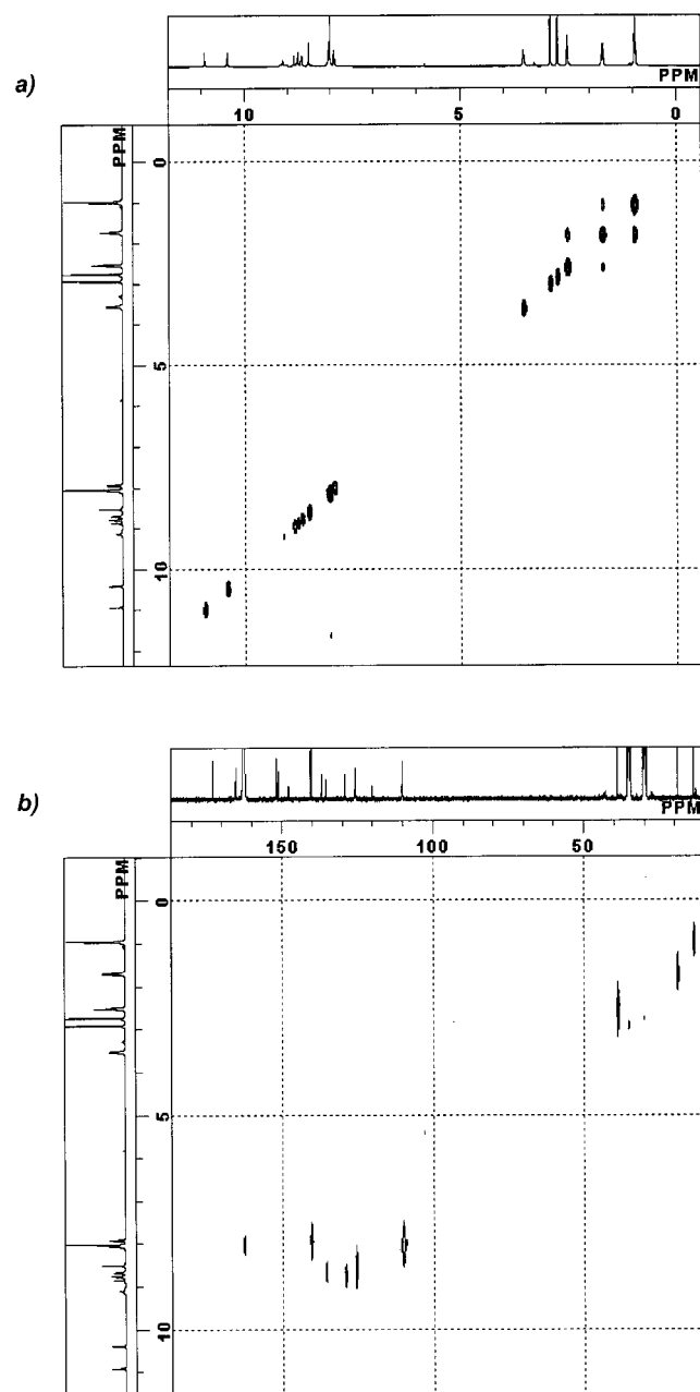
Figure 1. a) COSY and b) HETCOR NMR spectra of compound 1 (400 MHz, room temperature, [D_7] DMF).
